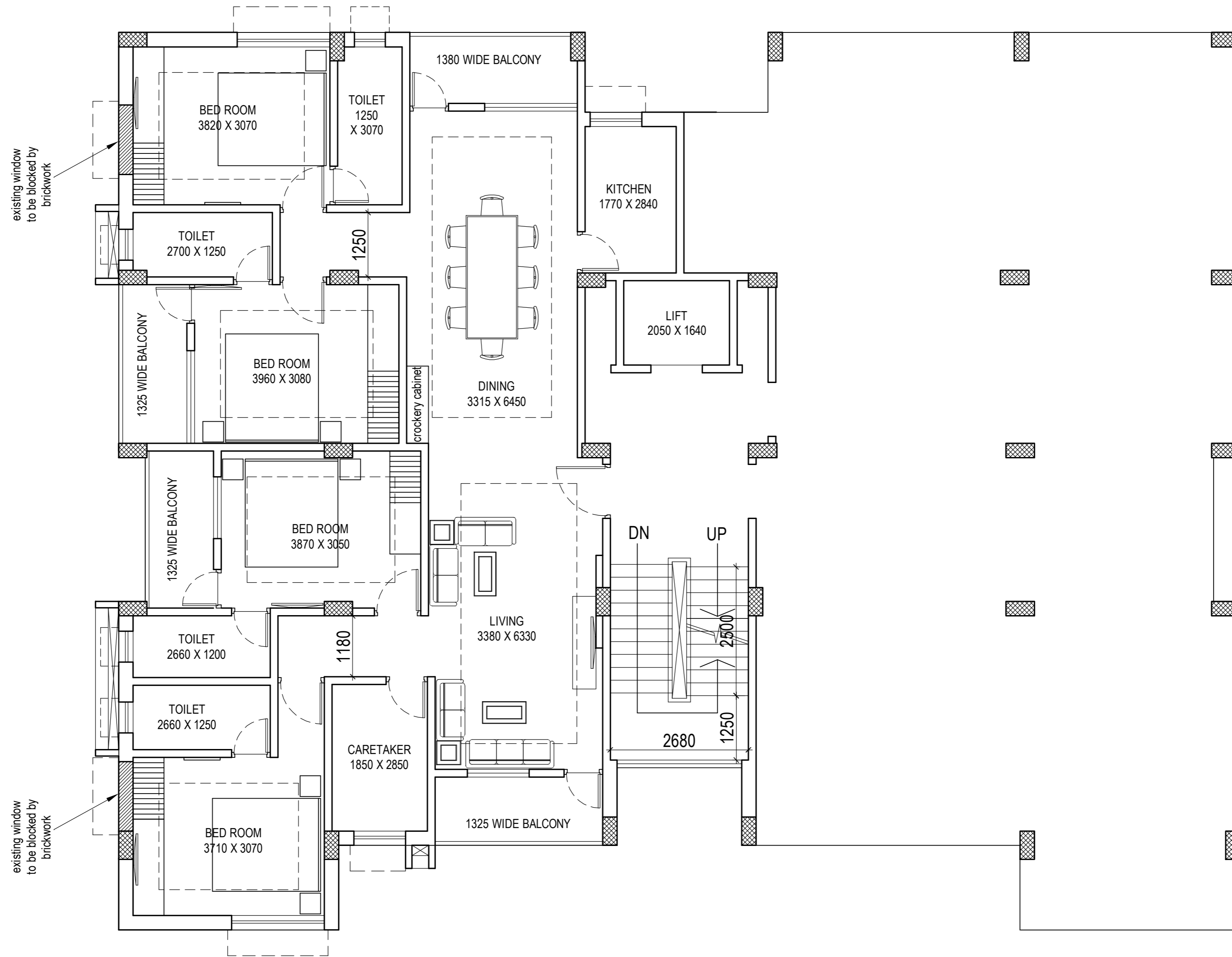
1ST FLOOR PLAN (GUEST HOUSE) OF BLOCK - A
