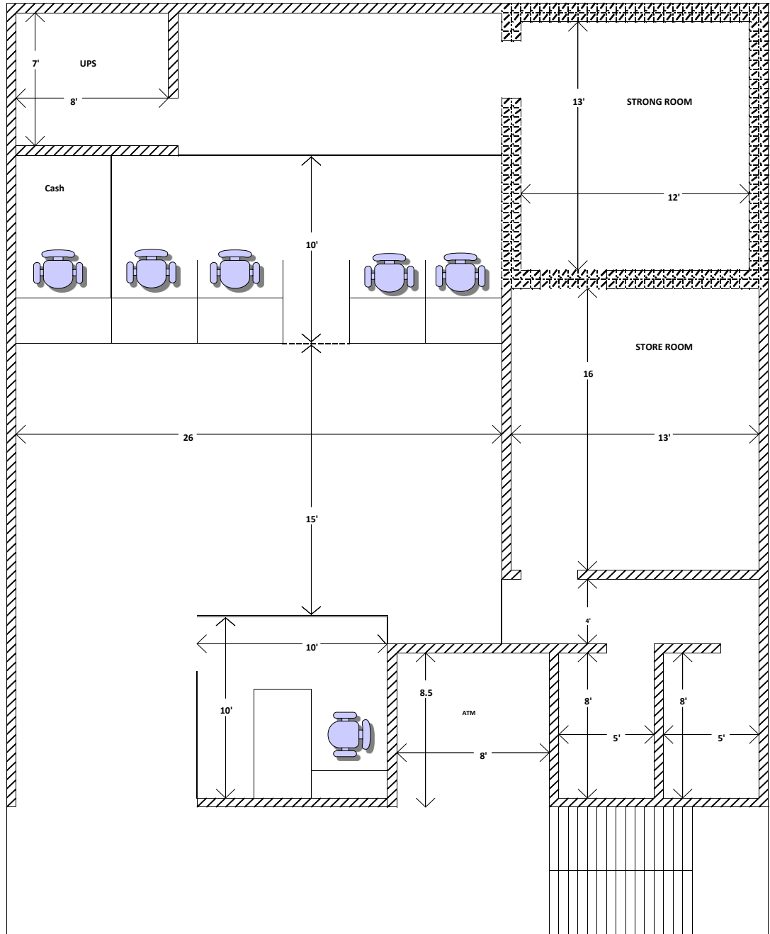
4501-KRISHNAPURAM PROPOSED LAYOUT
